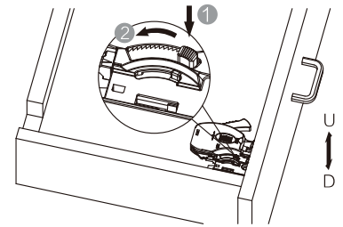
Height adjustment 0~+3mm
